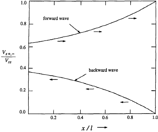
Fig. 2. Forward and backward waves on an exponential line.
