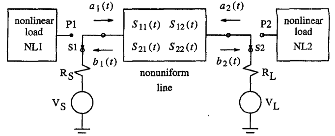
Fig. 3. Time-domain analysis and initial condition considerations.
