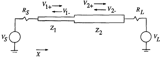
Fig. 1. Two traveling waves on a two-section line.
